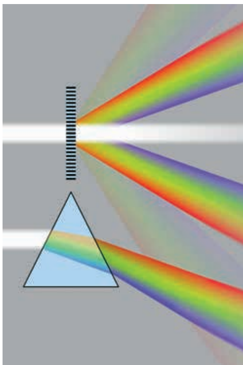
A diffraction grating (top) and a prism (bottom) will both separate white light into the visible spectrum.
